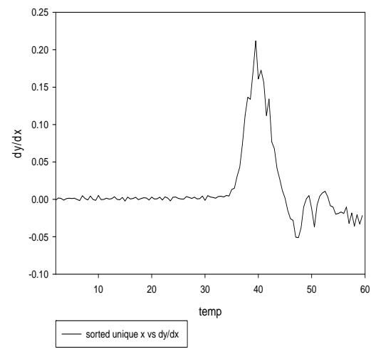
hNBD1WT110807 1st derivative of tmelt
