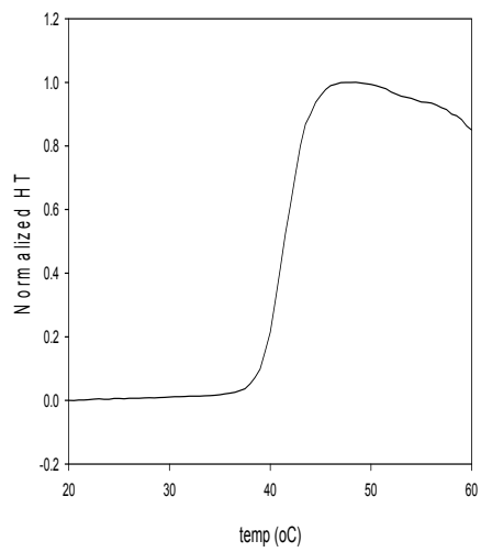
hNBD1wt062907 tmelt
