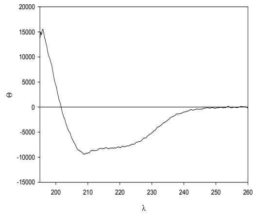
06-29-07 hwt mwpr molar ellipticity
