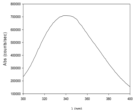
hNBD1wt062907 Fluorescence
